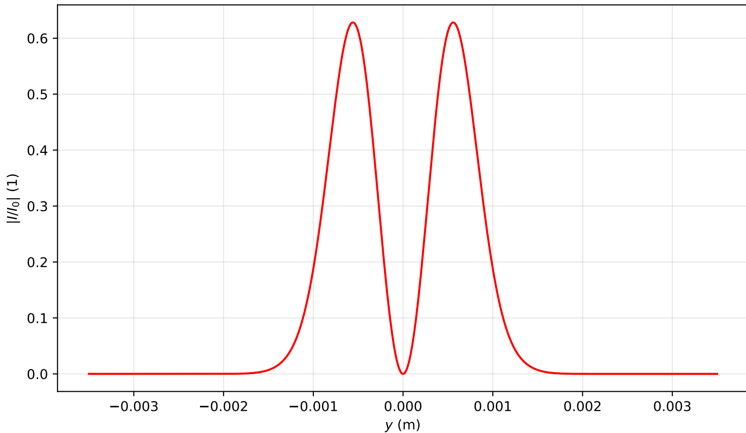
Intensity profile I(x=0, y, z=0.955)/I_0 , P_{in}=0.5P_{cr} , artificial time
